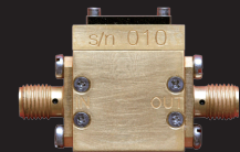
LNF-LNR4_14B (4GHz-14GHz/improved)
