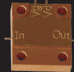
LNF-LNC15_29DRPA (15GHz-29GHz/drop-in)
