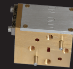
LNF-LNR65_115WB (65GHz-115GHz/waveguide)
