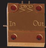
LNF-LNR15_29DRPA (15GHz-29GHz/drop-in)
