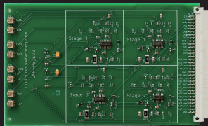
LNF-PS_EU2 (Constant current power supply for 1-4 LNAs)
